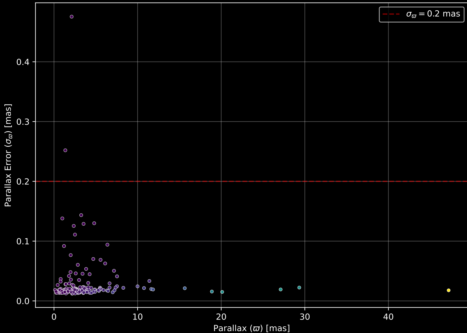
APOGEE DR17 Field: [174+35_MGA] Parallax Quality (n= 184)
