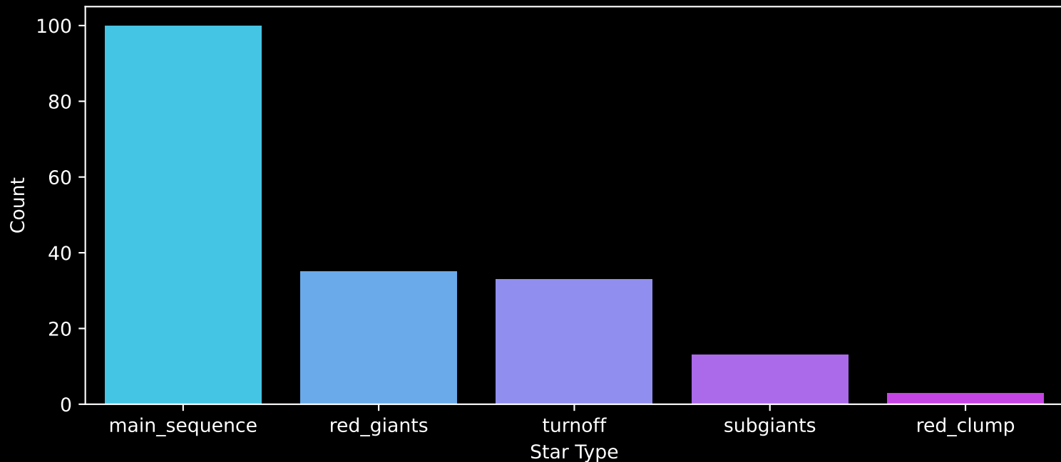
APOGEE DR17 Field: [174+35_MGA] Count plot of Star Type
