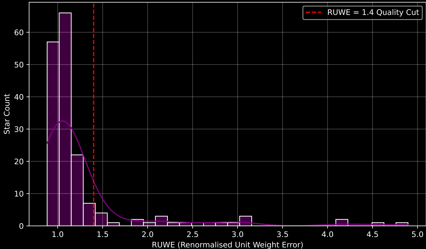
GAPOGEE DR17 Field [174+35_MGA] RUWE Distribution (n= 175)
