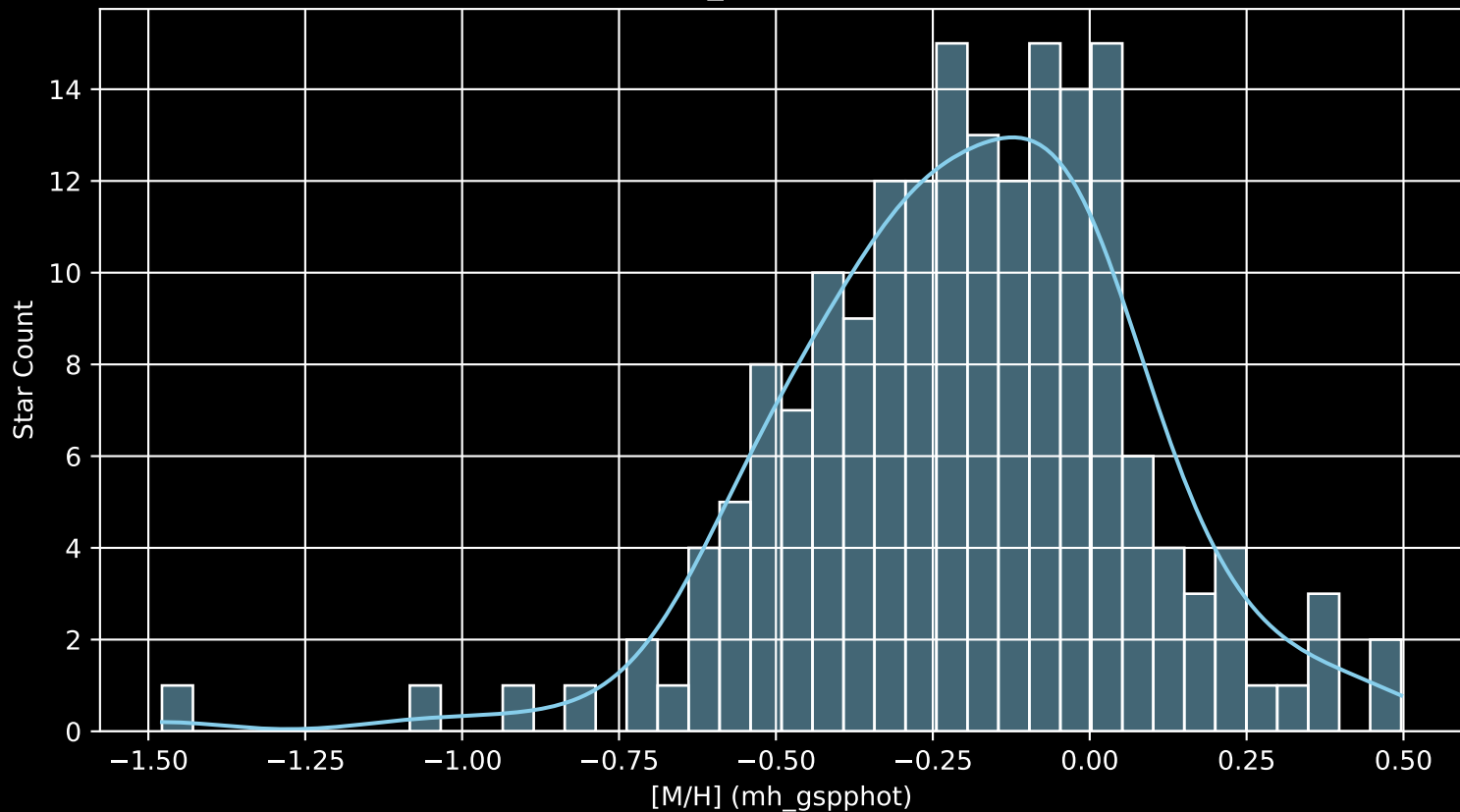
APOGEE DR17 Field: [174+35_MGA [M/H] (mh_gspphot) (n= 182)
