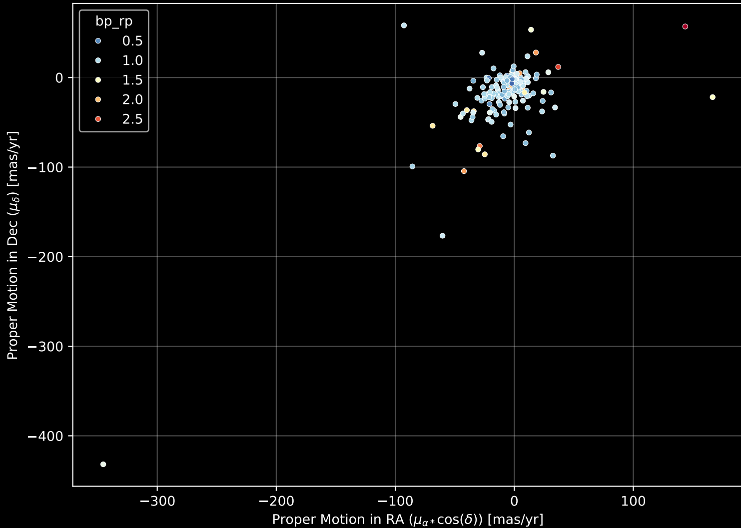
APOGEE DR17 Field: [174+35_MGA] Proper Motion Diagram (n= 184)
